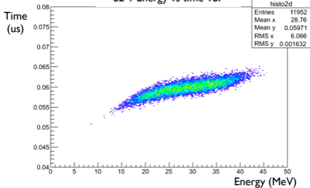
S2-I Energy vs time 21Ne
