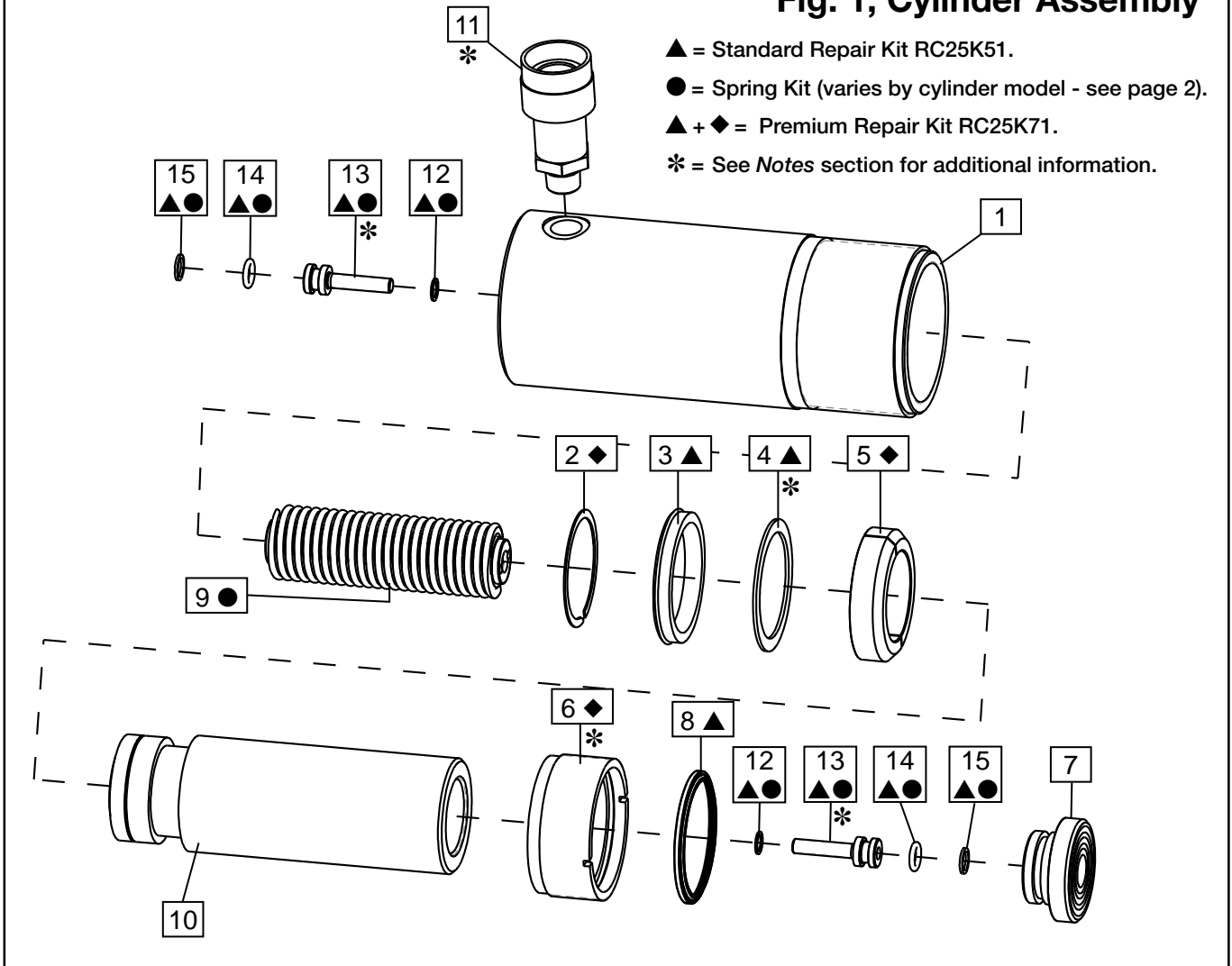
Fig. 1, Cylinder Assembly
