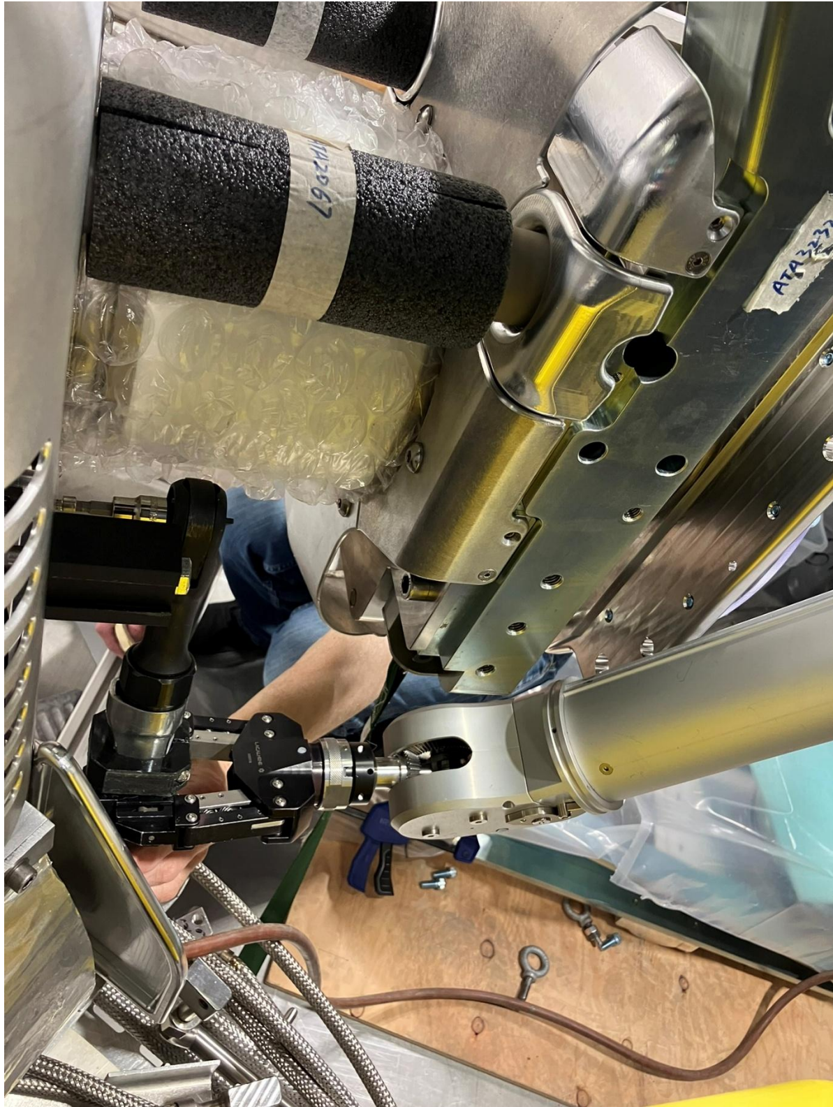
Tight clearance between manipulator wrist and driver side FE structure
