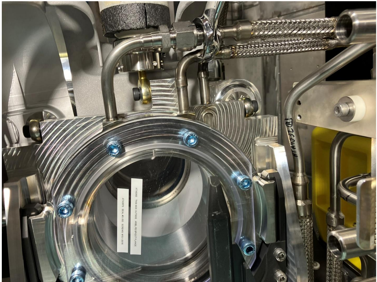
Wrench interference with adjacent line in second to top line's VCR joint
