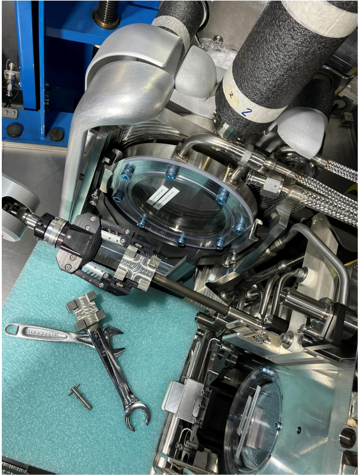
Use of pi detent tool to manipulate the water line without scratching the sealing face.
