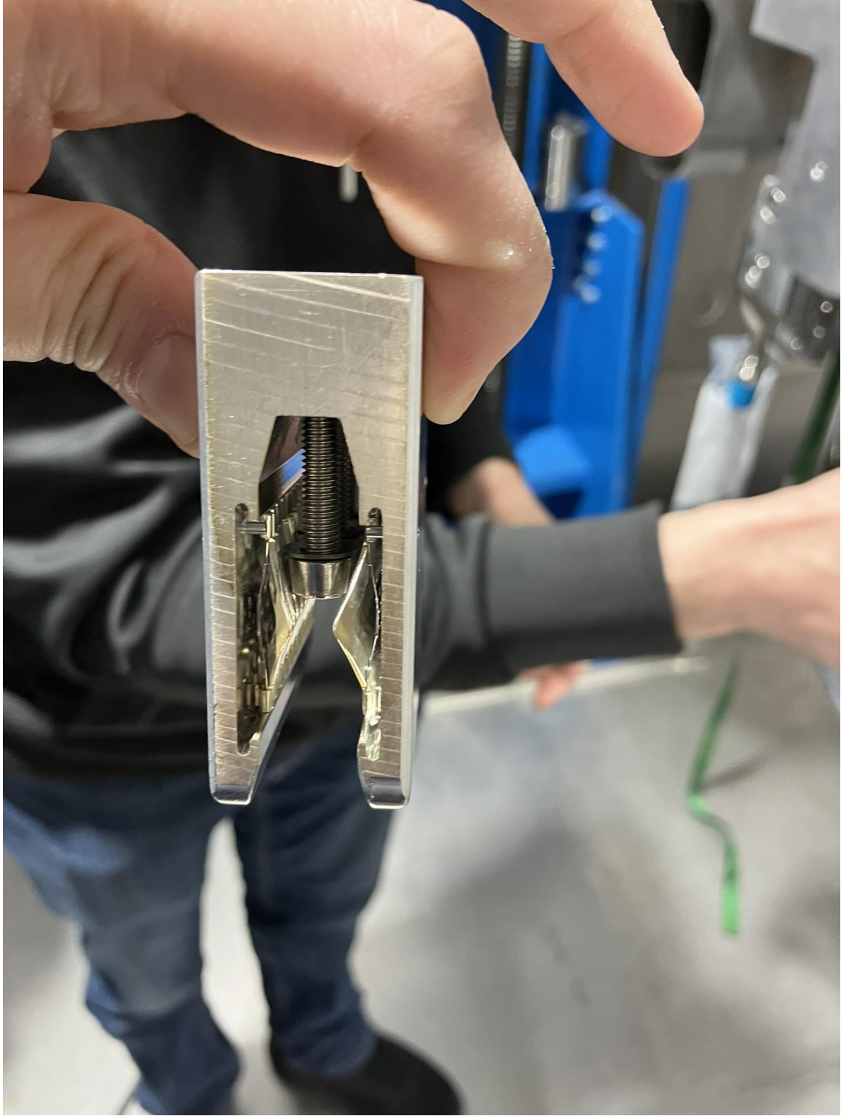
Screws captive in connector.
